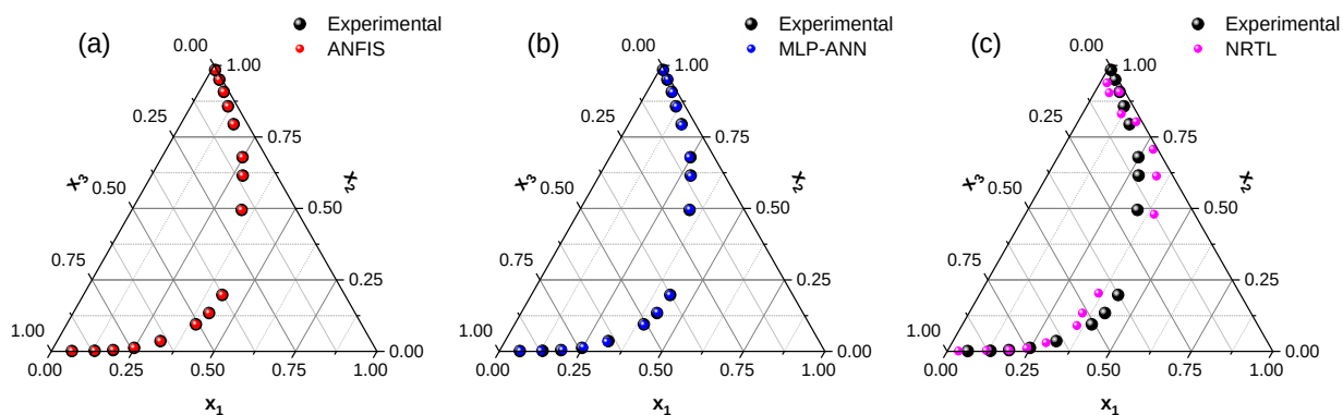
Fig. 2. Phase diagrams for the ternary system EtOH-benzene-water at 20 °C using a) ANFIS, b) MLP-ANN, c) NRTL
