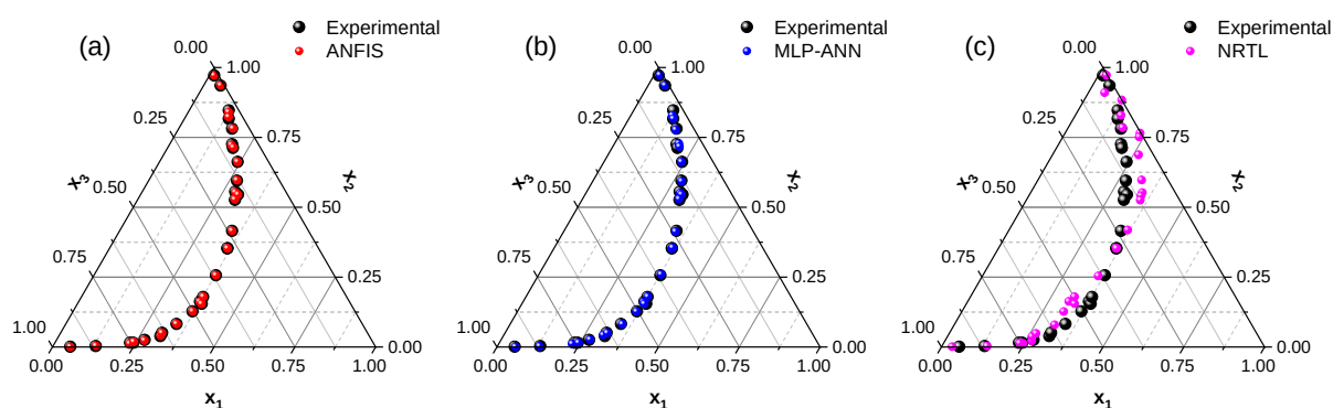
Fig. 3. Phase diagrams for the ternary system EtOH-benzene-water at 30 °C using a) ANFIS, b) MLP-ANN, c) NRTL
