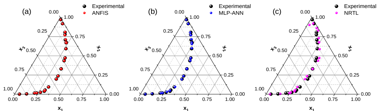
Fig. 4. Phase diagrams for the ternary system EtOH-benzene-water at 40 °C using a) ANFIS, b) MLP-ANN, c) NRTL
