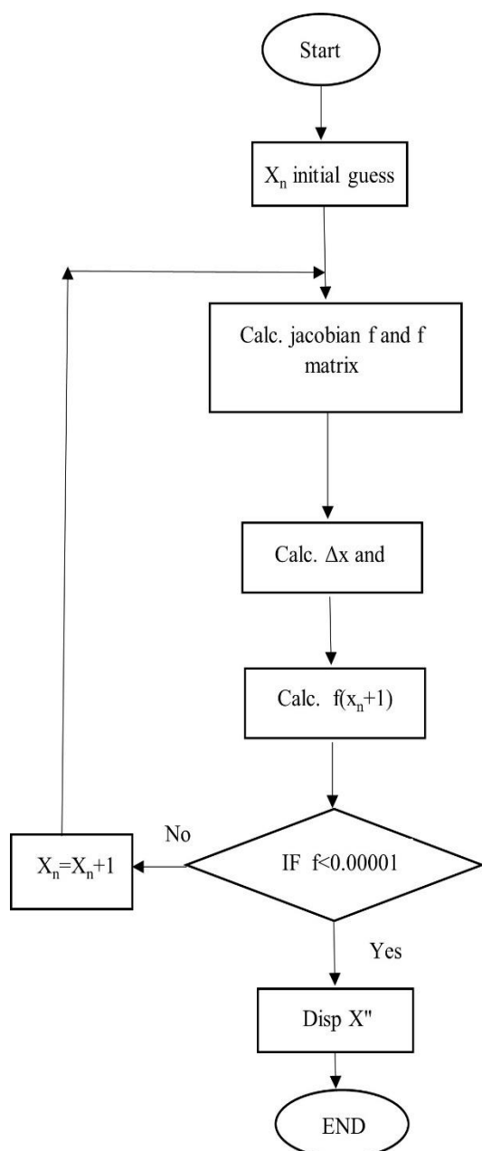
Fig. 1. Flowchart for solving sets of nonlinear equations using Newton's method
