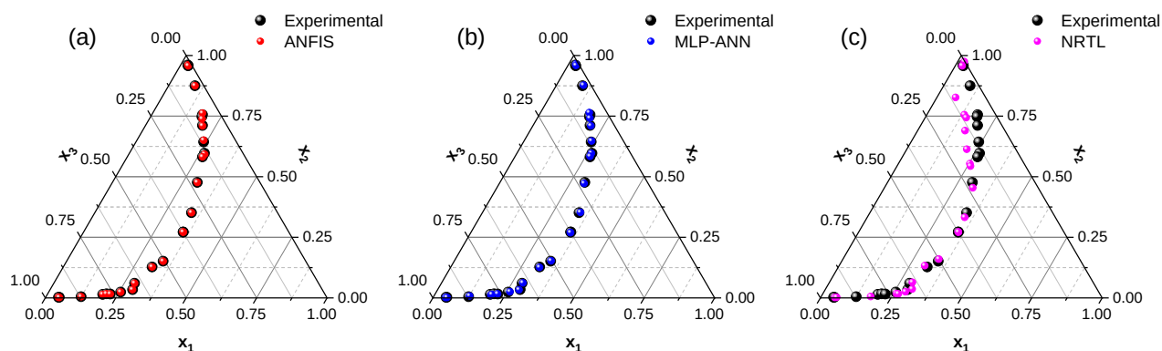
Fig. 5. Phase diagrams for the ternary system EtOH-benzene-water at 55 °C using a) ANFIS, b) MLP-ANN, c) NRTL
