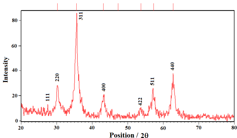
Fig. 1. XRD patterns of \text{AlCoFe}_2\text{O}_4
