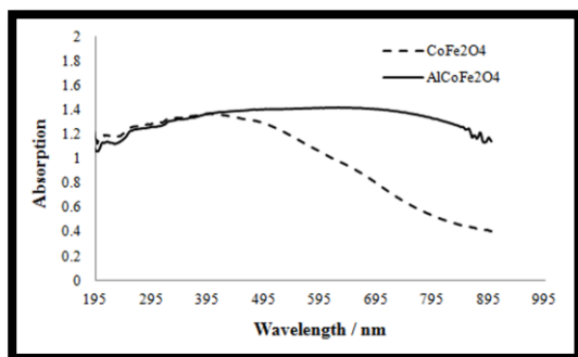
Fig. 6. UV-Vis spectra of \text{AlCoFe}_2\text{O}_4 and \text{CoFe}_2\text{O}_4 As can be seen, higher absorption of \text{AlCoFe}_2\text{O}_4 in the visible light region makes it possible to increase the photocatalytic performance of the photocatalyst under visible light irradiation.
