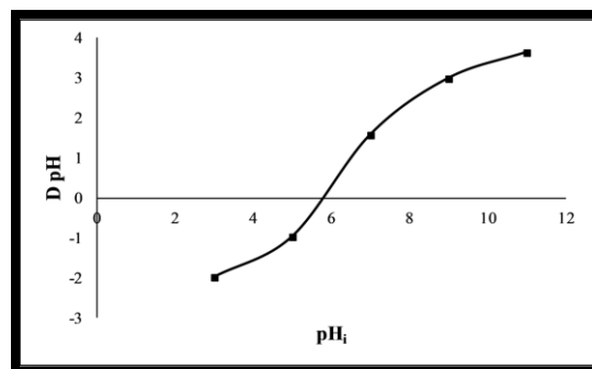
Fig. 7. Point of zero charge of \text{AlCoFe}_2\text{O}_4 nanocatalyst
