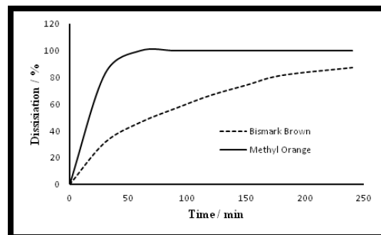
Fig. 9. Dissociation curve of MO and BB under UV irradiation.
