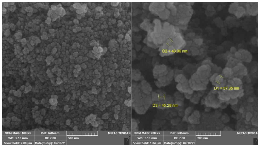
Fig. 3. FESEM image of \text{AlCoFe}_2\text{O}_4 nanocrystals
