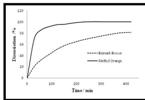
Fig. 10. Dissociation curve of MO and BB under Vis irradiation.
