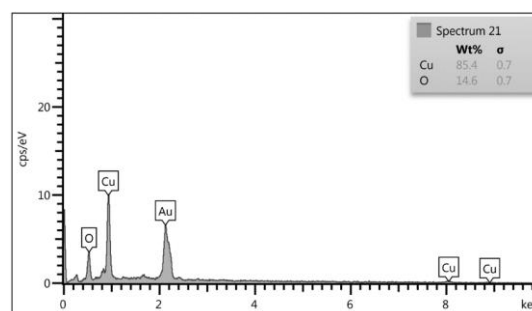
Figure 6. EDS analysis of CuO nanoparticles
