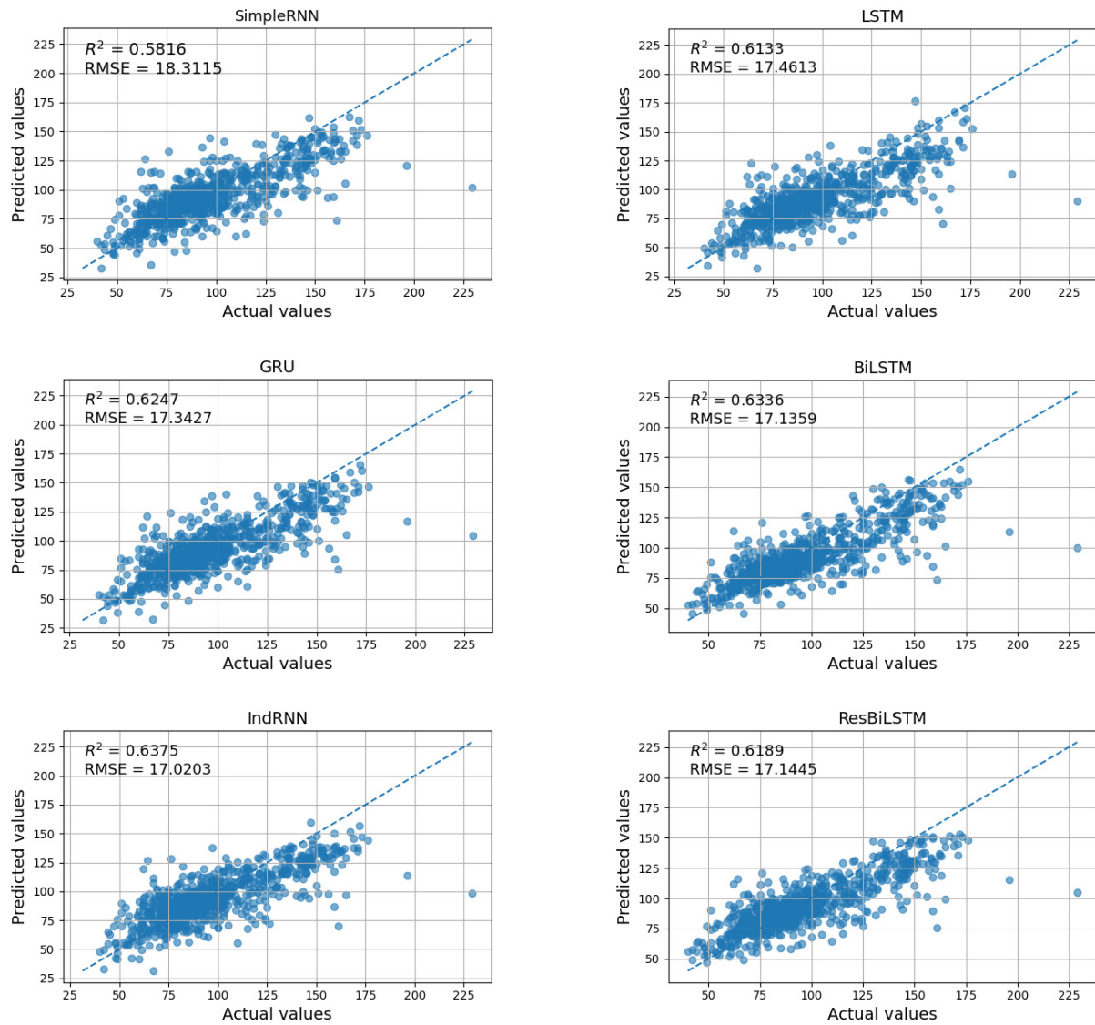
Figure 1: Scatter plots of the actual and predicted pollutant concentrations
