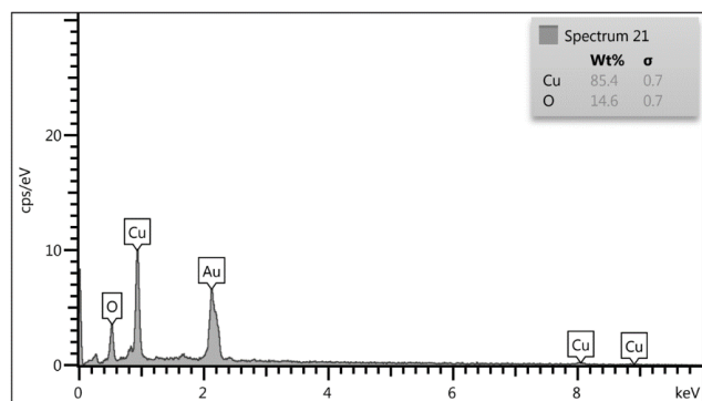
Figure 6. EDS analysis of CuO nanoparticles
