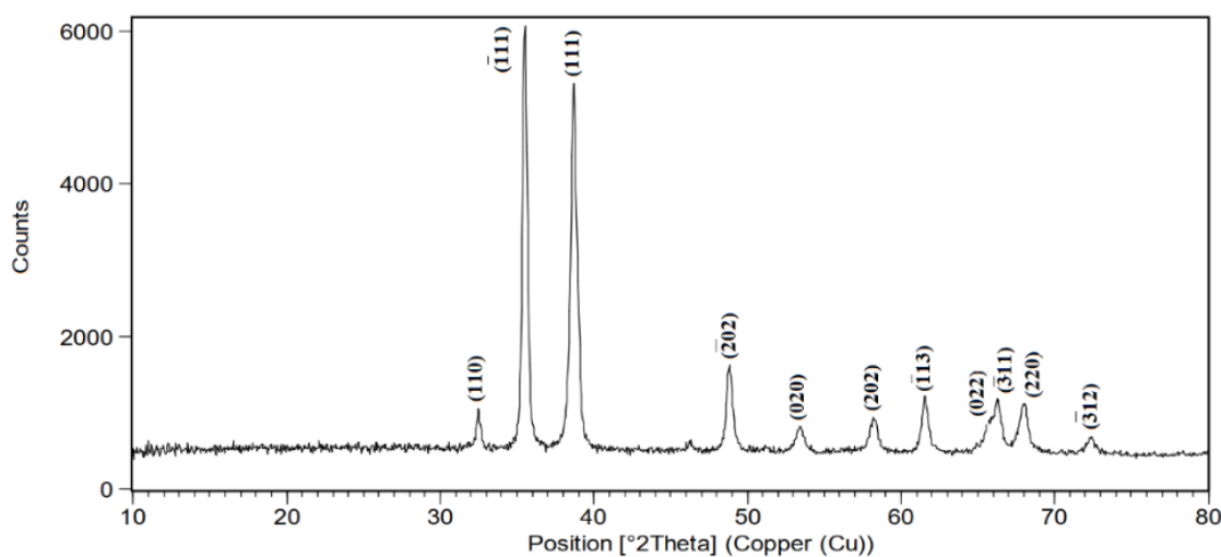
Figure 4. The XRD patterns of CuO nanoparticles
