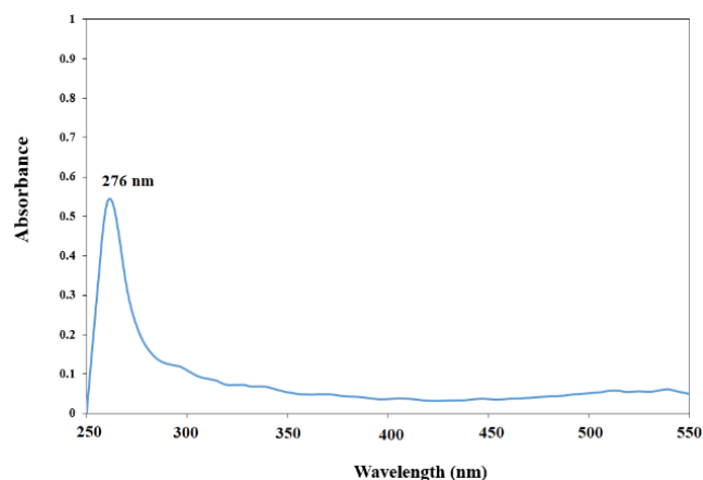
Figure 7. The UV-Vis spectra of CuO nanoparticles
