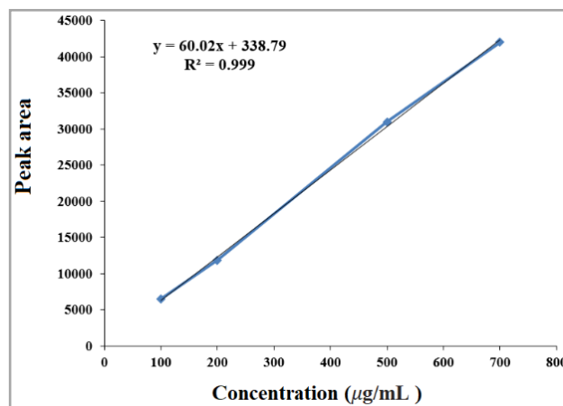
Fig. 2. Calibration curve of 5-FU
