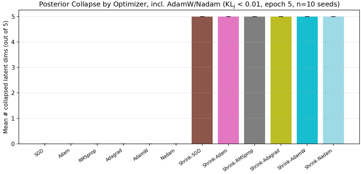
Figure 3: Posterior collapse diagnostic (mean number of latent dimensions with KL_j < 0.01 at epoch 5, out of 5) for all twelve optimizers, including AdamW and Nadam, mean \pm std over 10 seeds. Every shrinkage-augmented optimizer collapses all 5 latent dimensions in every seed; no non-shrinkage optimizer collapses any dimension.
