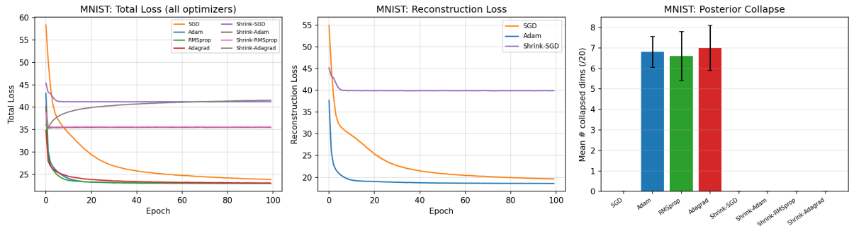
Figure 4: MNIST at \alpha = 10^{-3} (mean \pm std, 5 seeds, 5,000 training images). Left : total loss, all eight base optimizers over 100 epochs (AdamW/Nadam, not shown, track Adam almost exactly). Middle : reconstruction loss, Adam vs. SGD vs. Shrink-SGD. Right : posterior-collapse diagnostic (mean # of 20 latent dimensions with KL_j < 0.01 at epoch 100). This pattern is not robust to changes in learning rate or architecture, see Section 6.3.
