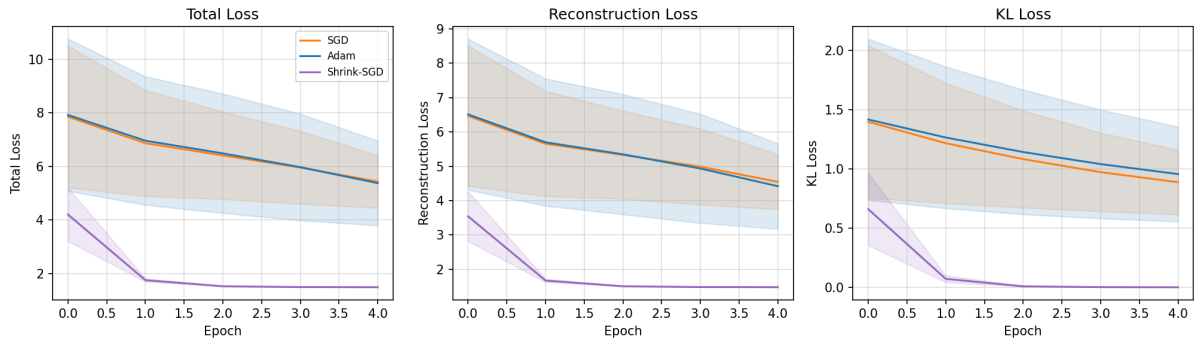
Figure 2: Total, reconstruction, and KL loss for SGD, Adam, and the Shrinkage Optimizer (mean \pm std, 10 seeds).
