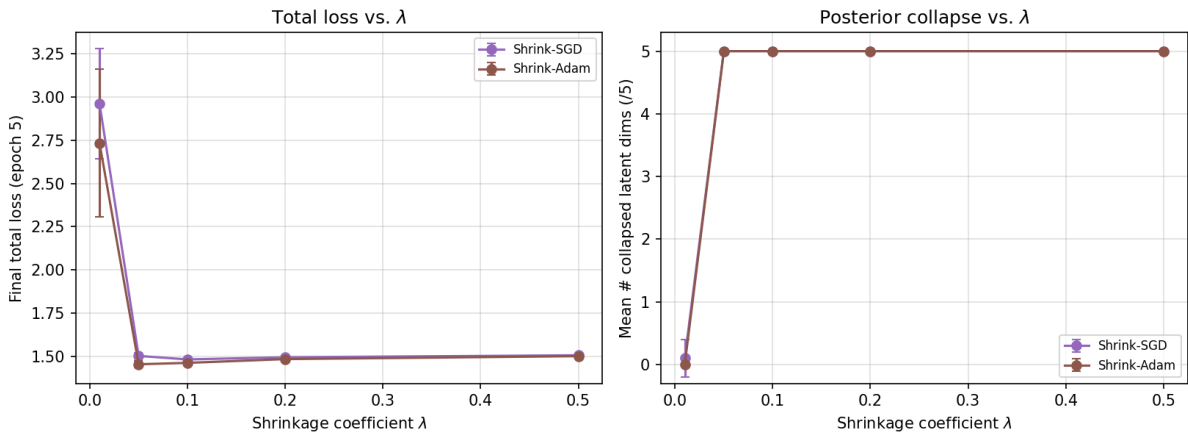
Figure 6: Sensitivity of the synthetic-dataset results to the shrinkage coefficient \lambda (Shrink-SGD and Shrink-Adam, mean \pm std over 10 seeds). Left : final total loss. Right : mean number of collapsed latent dimensions (out of 5). A sharp collapse threshold appears between \lambda = 0.01 and \lambda = 0.05 .
