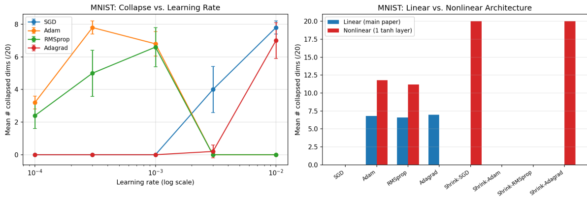
Figure 7: MNIST robustness checks (linear architecture unless noted, mean, 5 seeds). Left : posterior collapse vs. learning rate, no optimizer is uniformly resistant; Adam/RMSprop’s collapse is non-monotonic and returns to zero at higher \alpha , while SGD’s collapse increases with \alpha . Right : linear vs. nonlinear architecture at \alpha = 10^{-3} , Shrink-SGD and Shrink-Adagrad go from zero to complete collapse; Adagrad goes from substantial to zero collapse; Adam and RMSprop’s collapse roughly doubles.
