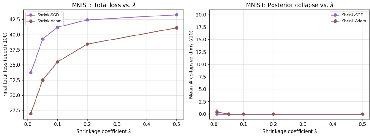
Figure 5: MNIST: sensitivity to the shrinkage coefficient \lambda for Shrink-SGD and Shrink-Adam (mean \pm std, 5 seeds, linear architecture). Unlike the synthetic dataset (Figure 6), no sharp collapse threshold appears; collapse remains at zero across the full range tested.
