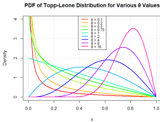
Figure 1: Graphical representation of PDF for the TL Distribution with varying \theta values.
