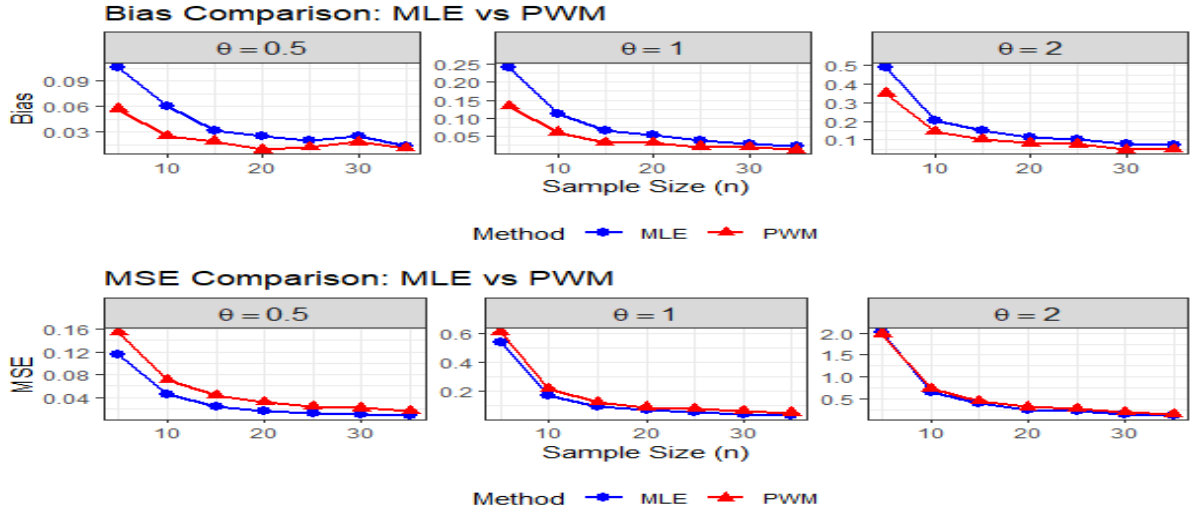
Figure 3: Comparing Bias and MSE for MLE and PWM across sample sizes, with separate lines for \theta = 0.5, 1.0, 2.0 .
