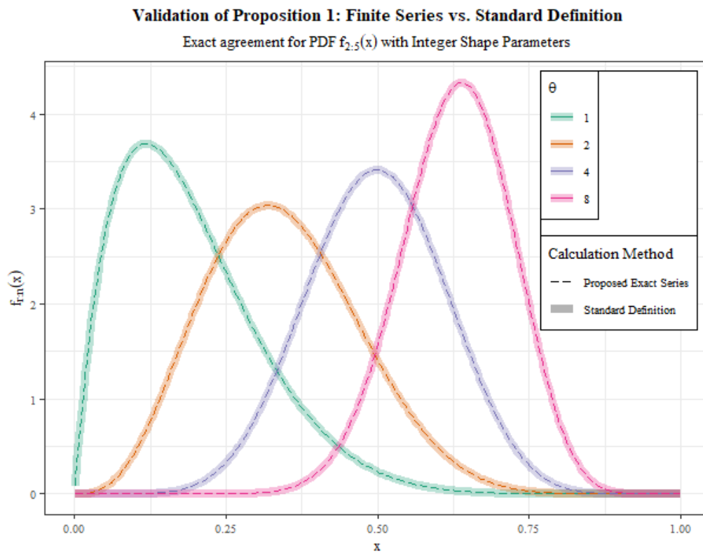
Figure 4: n = 5, r = 2 . The dashed lines (representing the derived formula in Eq. 7) strictly coincide with the thick solid lines (representing the standard definition), confirming the exactness of the finite series representation for integer \theta .
