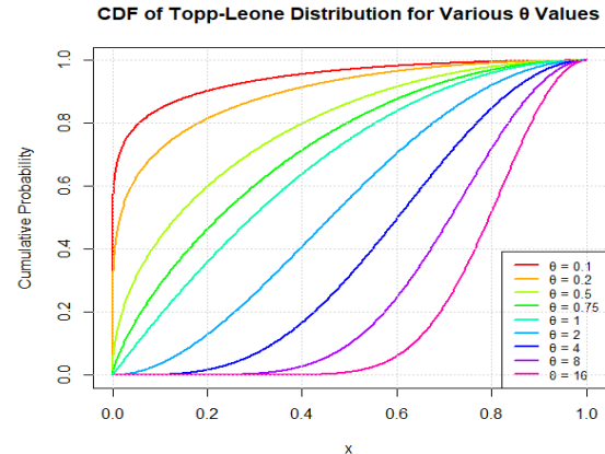
Figure 2: Graphical representation of CDF for the TL Distribution with varying \theta values.
