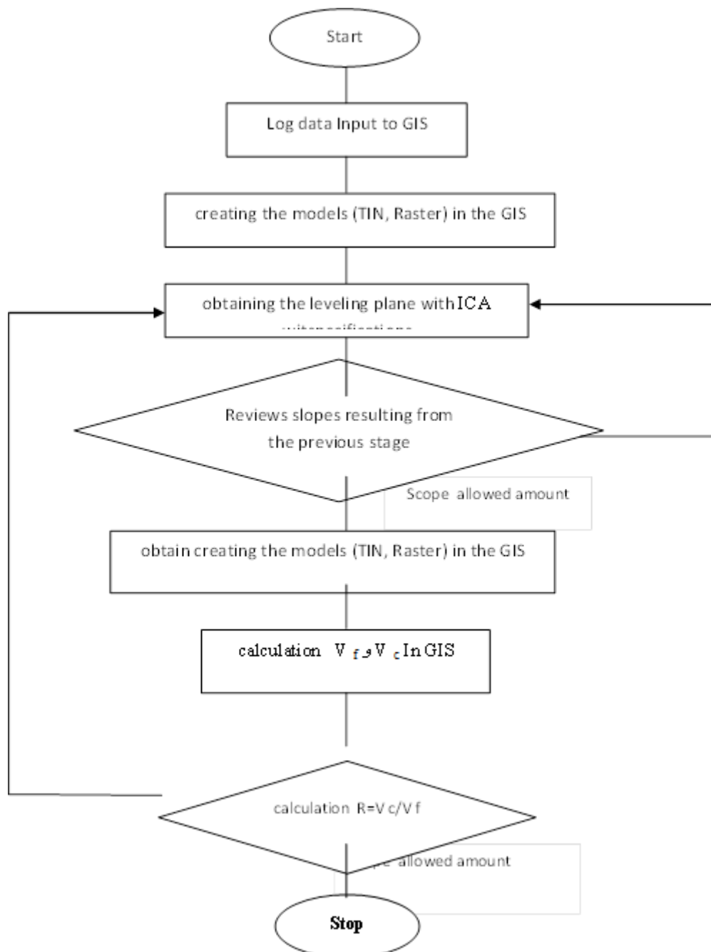
Figure 3) The suggested method in this research.
