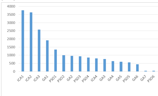
Figure 8) Cost saving in energy consumption for different models (Thousand Rials).
