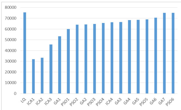
Figure 7) Volume of earthworks at different methods (M3).
