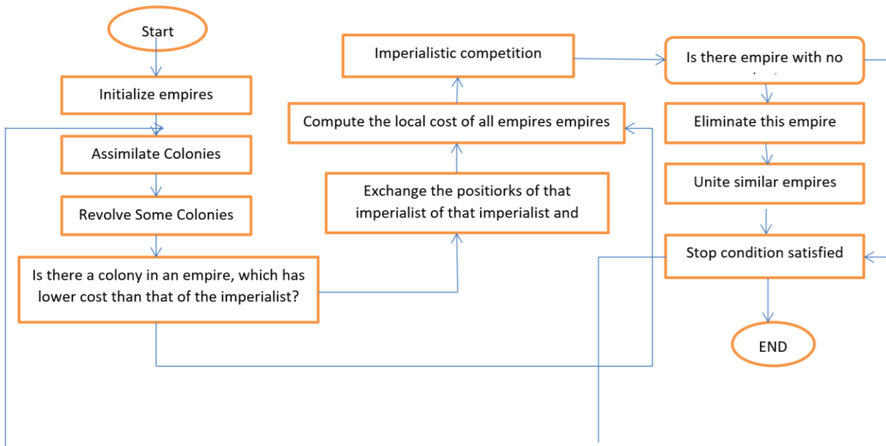
Figure 4) Flowchart of the imperialist competitive algorithm.
