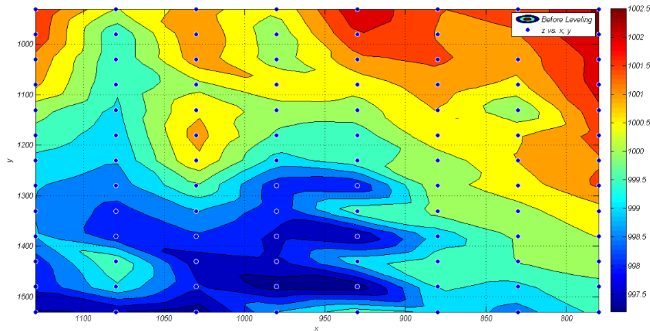
Figure 2) Map Contour map of the topography of the land before leveling.
