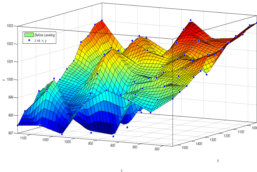
Figure 1) Schematic of the topography of the land before leveling experiment.
