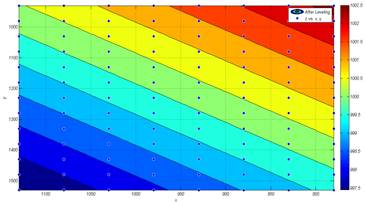
Figure 6) Map leveling of ground at different levels by ICA.
