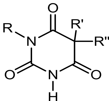
Figure 1. The structural template of barbiturates
