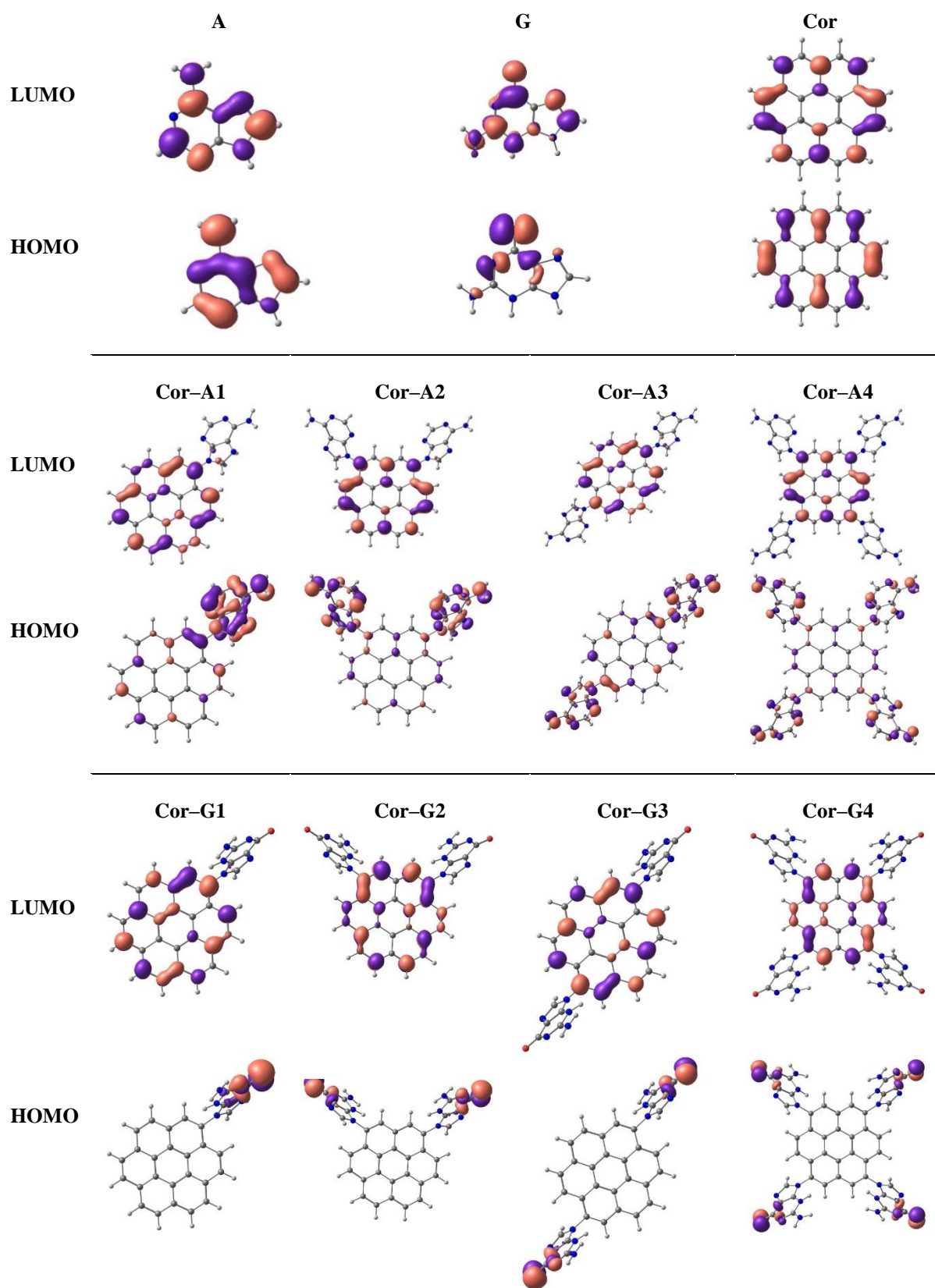
Figure 2. HOMO and LUMO distribution patterns for Cor, A and G singular models and Cor-P hybrid models
