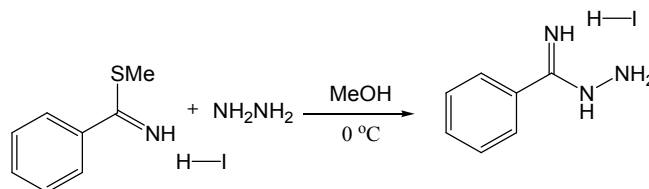
Scheme 1. Synthesis of benzamidrazone hydroiodide
