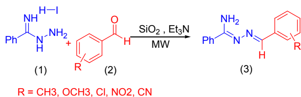
Scheme 2. Microwave-assisted synthesis of aminoazines
