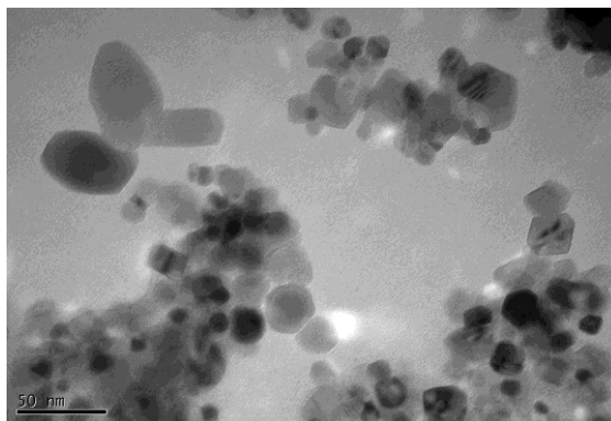
Figure 3. TEM image of \text{Co}_3\text{O}_4 nanoparticles
