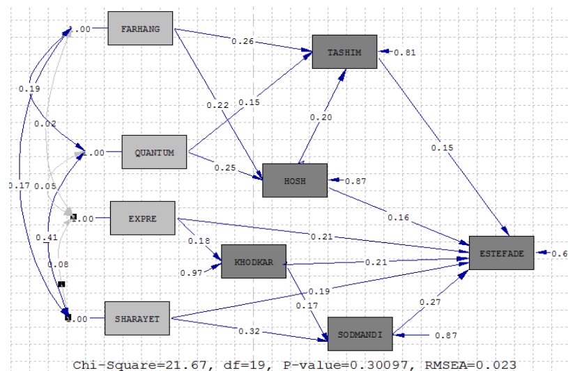
Fig 1. Path diagram and the estimated parameters of the fitted model (direct effects)
